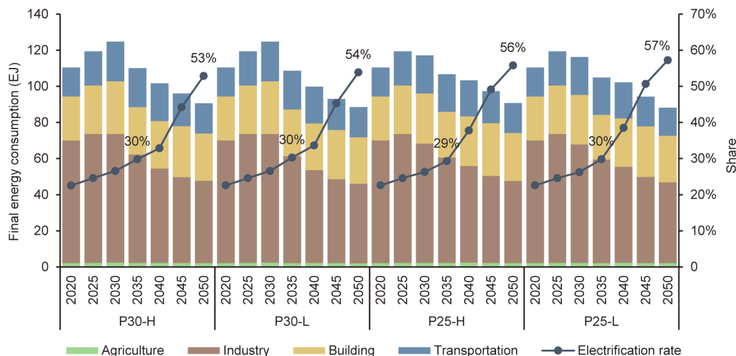
Fig. 5. Final energy consumption by sector and the electrification rate.
